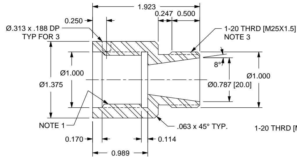
1 HOLDER mat'l - steel 1 required
